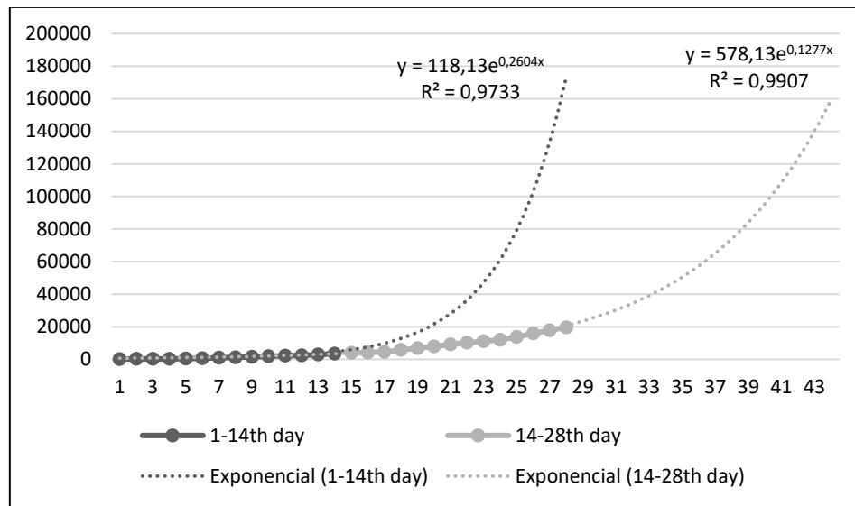
FIGURE 2: Historical series of COVID-19 cases in Brazil after detected 100 cases, 2020. Fonte: Worldometers (2020).
